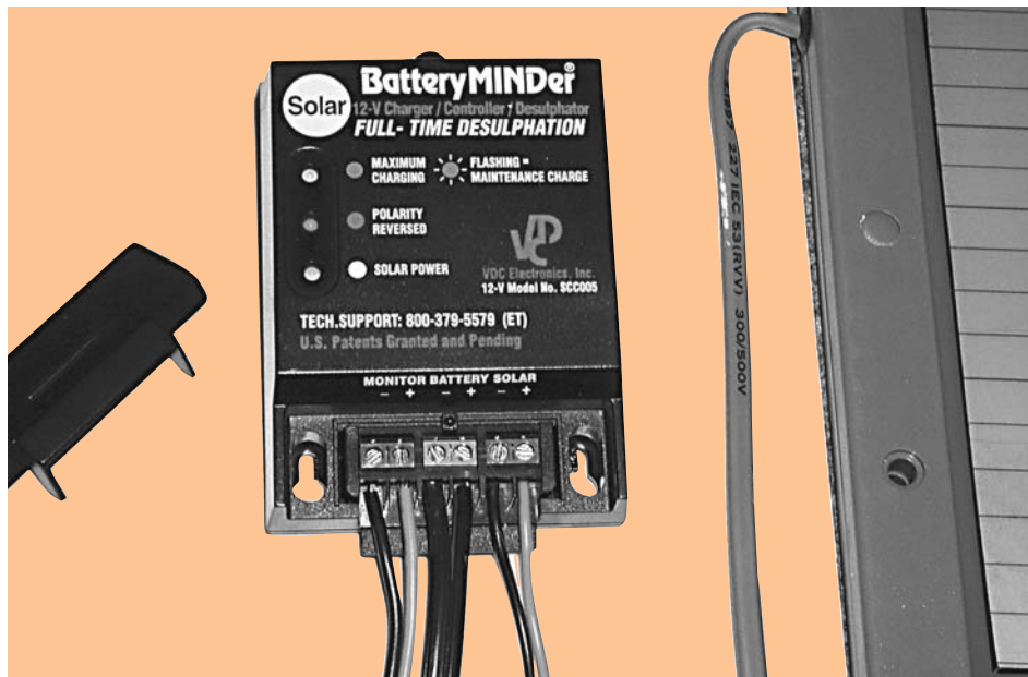
— + To Solar Panel
