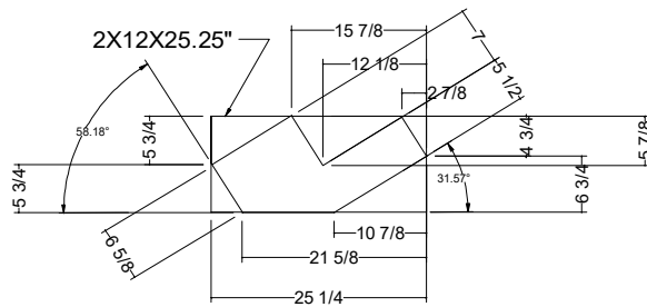
Stringer Dimensions
